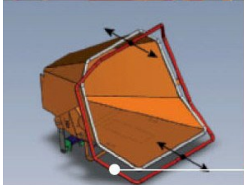
Optimum operator safety system: safety bar wrapped around the entire infeed funnel (VANDAELE® patent)
